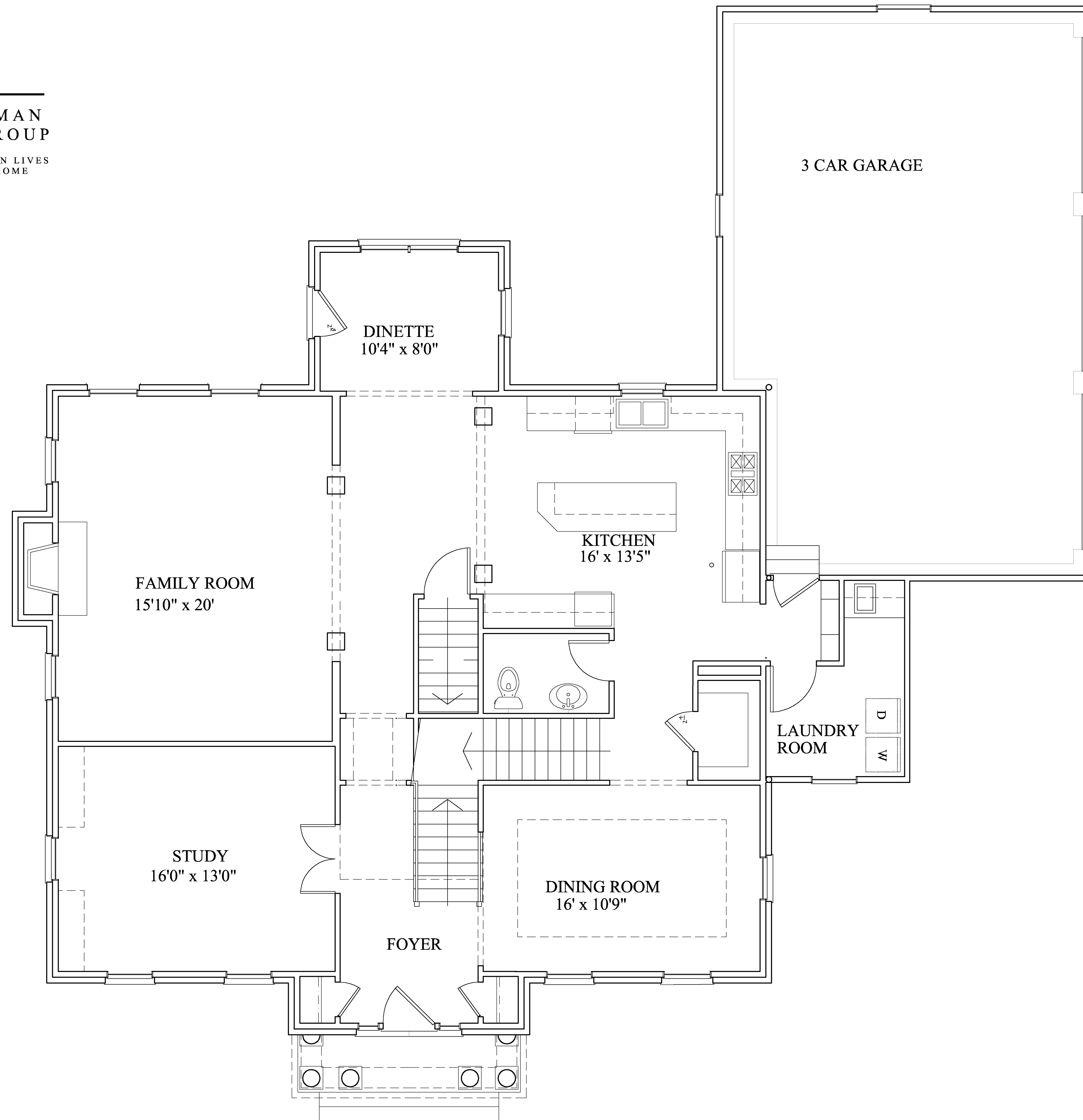
FIRST FLOOR PLAN LOT 2 Erye Hall
